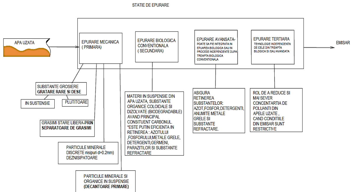
Diagrama flux SEAU
